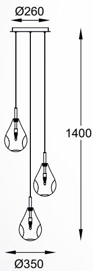
BASTONI new Pendant lamp MD1921-3B-CLEAR 3xG9 MAX 40W metal chrome body and canopy, clear glass shade
