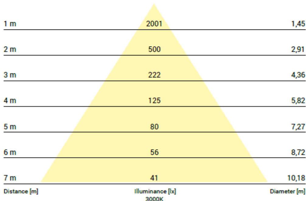
Beam cone diagram Beam angle 65°
