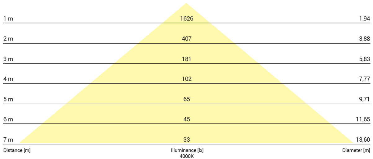
Beam cone diagram Beam angle 90°
