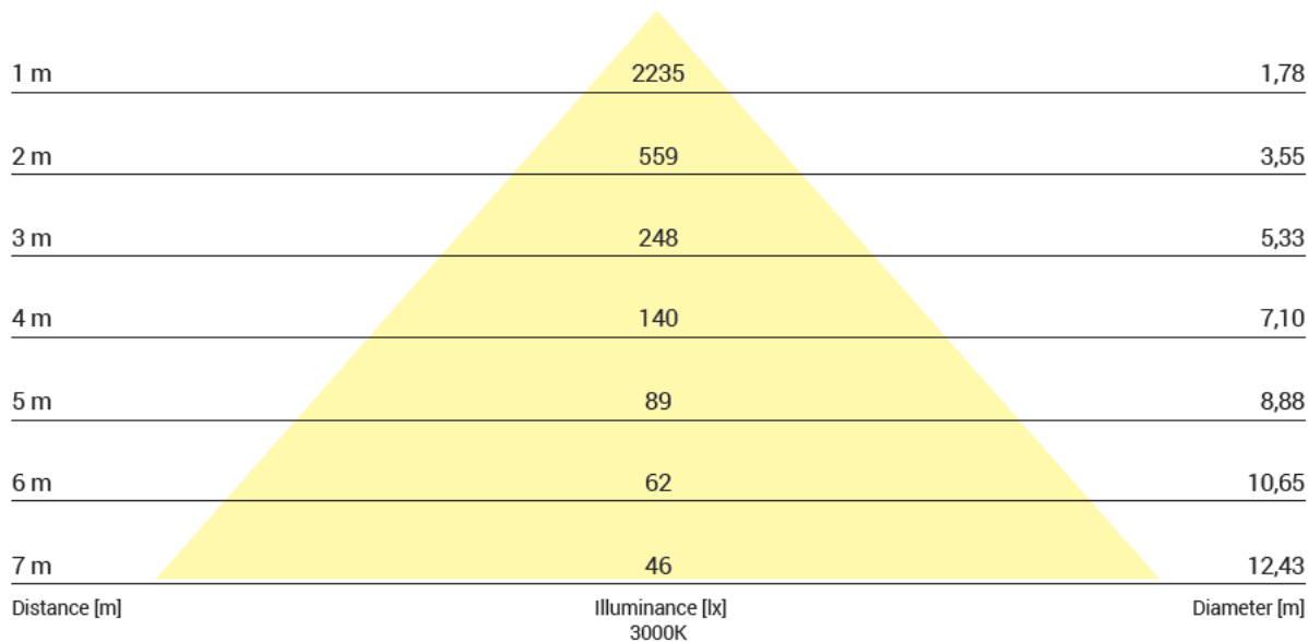
Beam cone diagram Beam angle 83°
