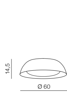
LED Lenox Top 60 AZ3146 (black/copper) LED 40W 3280lm 3000K aluminium/acrylic
